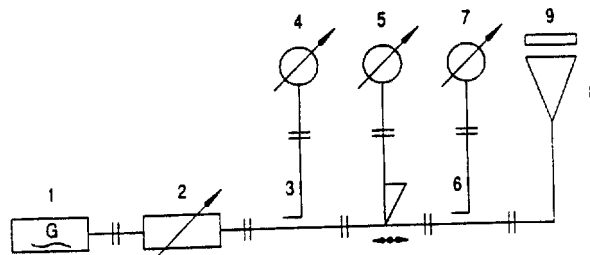
Fig. 1. Block diagram for microwave irradiation of cell suspension: 1 - EHF EMR generator; 2 - controlled attenuator; 3, 6 - directional coupler; 4 - frequency analyzer; 5 - measurement coupler; 7 - power meter; 8 - pyramidal horn; 9 - cell suspension.
