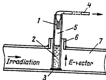
FIG. 2. Arrangement of tube with liquid in waveguide and bimorphous crystal in tube: 1 - detector of mechanical vibrations (bimorphous crystal); 2 - test liquid; 3 - packing (fluoroplast); 4 - coaxial cable; 5 - test tube; 6 - tube; 7 - waveguide.
