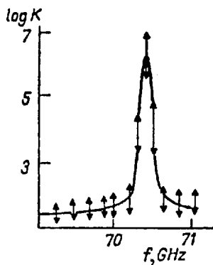
FIG. 1. Induction coefficient of lambda prophage as a function of the frequency of the acting radiation [11].
