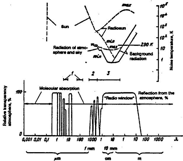
Fig. 1. Natural EMF sources and atmospheric transparency throughout the EM spectral range [12]: 1) frequency "windows" in which BII are observed according to [5]; wavelength bands where biological effects of nonthermal EMF with FD \leq 1 \text{ mW/cm}^2 can be observed; 2) data of [7]; 3) data of [1,3,10,13].
