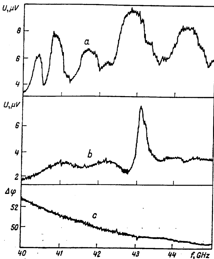
Frequency dependence of absorption of the energy of modulated mm emission impinging on: a —rectangular quartz cuvette (1 mm thick) filled with water and positioned in the near zone of the horn ( U is the signal of the piezo detector at the rear wall of the cuvette); b —polyethylene capillary (internal diameter 0.7 mm) with water passing through the waveguide ( U is the signal of the microphone inserted into the capillary at a distance 1 cm from the waveguide); c —is the skin of the human hand (between the horn and the skin is a well harmonizing fluoroplast gas microphone cell: \Delta\phi is the phase shift between the modulating and acoustic signals).
