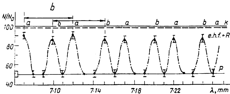
FIG. 2. Dependences of the normalized growth rate of a yeast culture on the frequency of the acting radiation [12] (a) and change in the number of karyocytes ( N/N_0 ) after exposure to e.h.f. combined with X-radiation with the wavelength of e.h.f. radiations in free space [19] (b).
