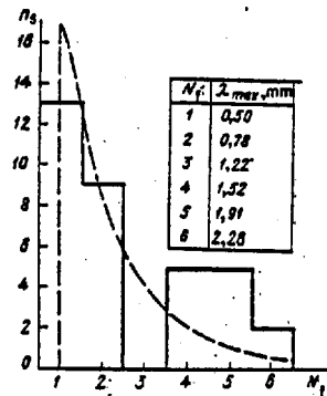
Fig. 6. Distribution of occurrence frequency of sensory reactions with BII through filters with various transmittance maxima.
